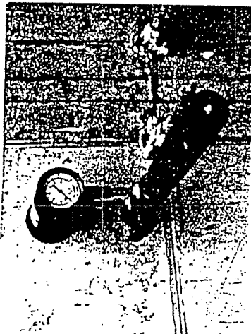
Fig.13. Testing of bottom slab with LOK-TEST and COMA-Meter.
