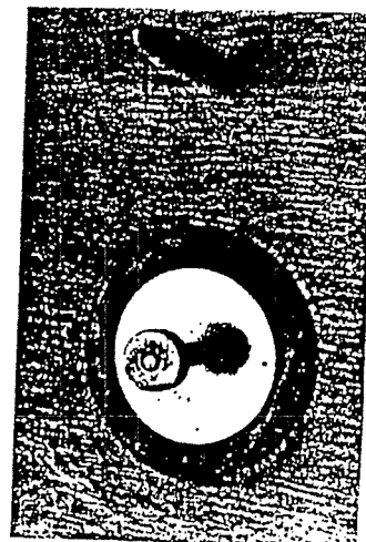
Fig. 18. LOK-TEST L-42 insert with L-44 steelplate installed in slab formwork together with one COMA-Meter (seen from casting side).
