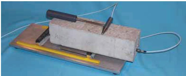
Specimen supported on test bench for measurement of longitudinal resonant frequency. Specimen is struck at end opposite to transducer position.
